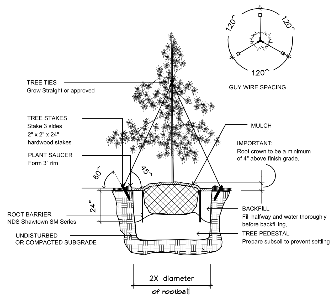
CONIFEROUS TREE PLANTING DETAIL
